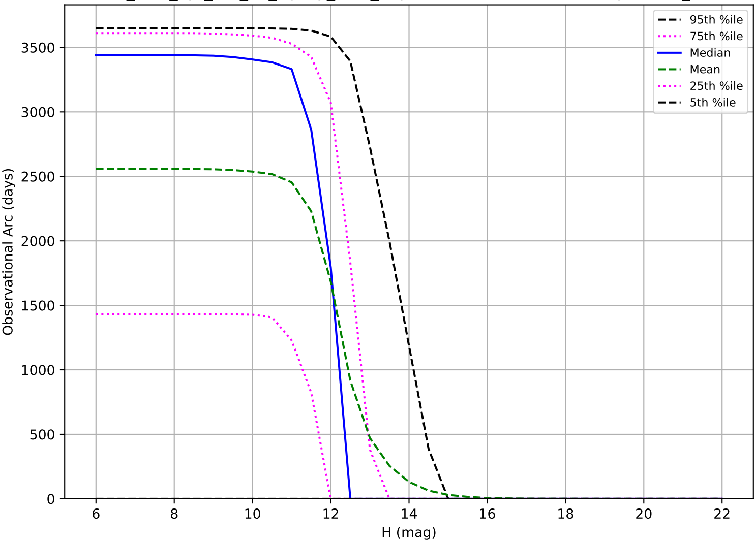
too_elab_2yr_r64_d3_ugrizy_v3.4_10yrs: Observational Arc Length OCC_r20
