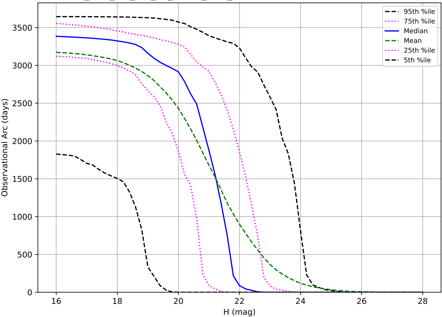
too_elab_2yr_r64_d3_ugrizy_v3.4_10yrs: Observational Arc Length NEO
