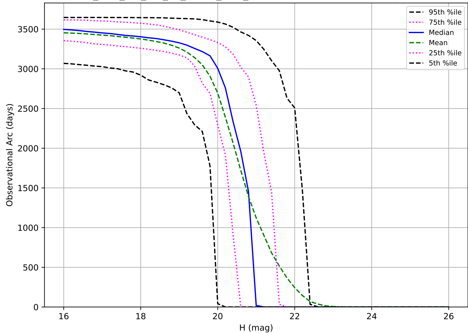
too_elab_2yr_r64_d3_ugrizy_v3.4_10yrs: Observational Arc Length MBA
