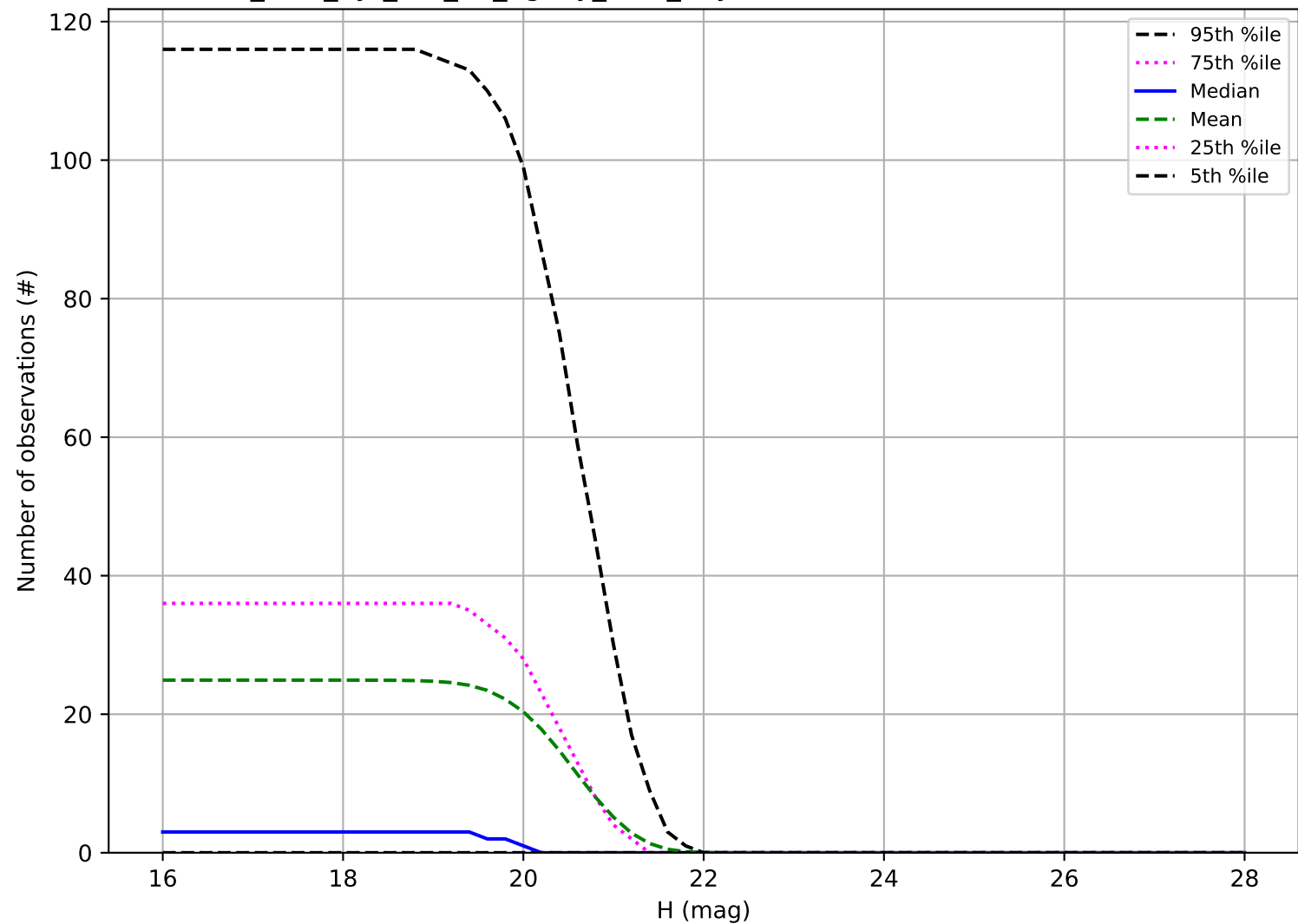
too_elab_2yr_r64_d3_ugrizy_v3.4_10yrs: Number of observations Vatira
