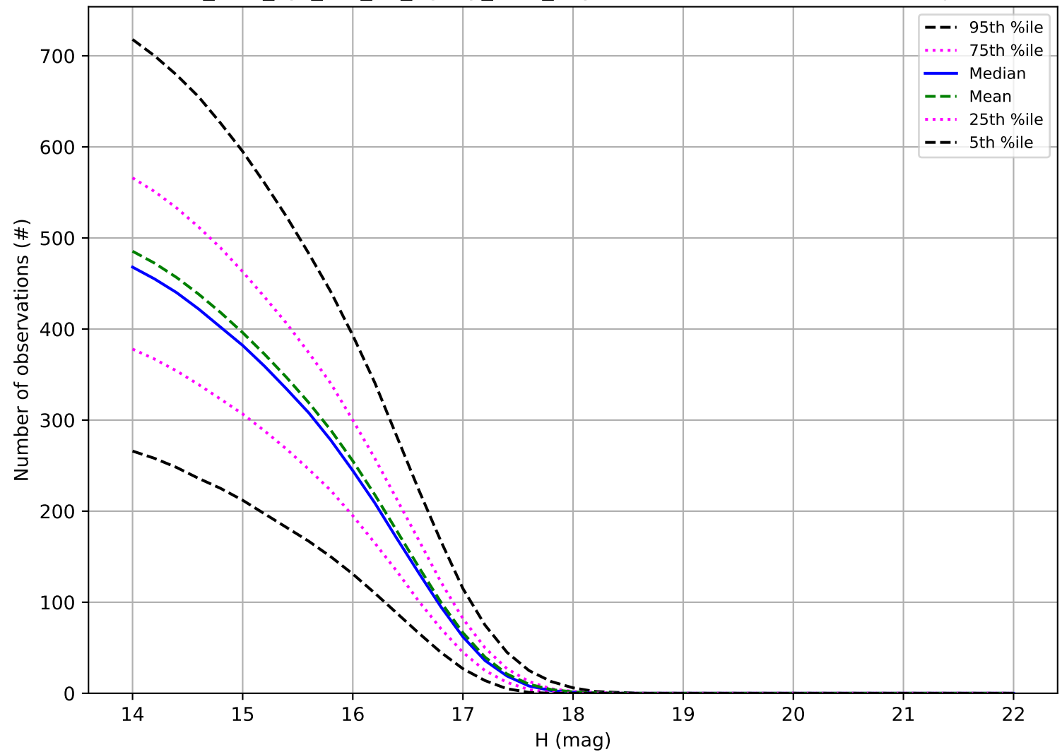
too_elab_2yr_r64_d3_ugrizy_v3.4_10yrs: Number of observations Trojan
