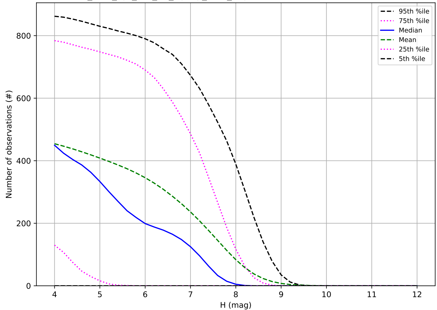
too_elab_2yr_r64_d3_ugrizy_v3.4_10yrs: Number of observations TNO
