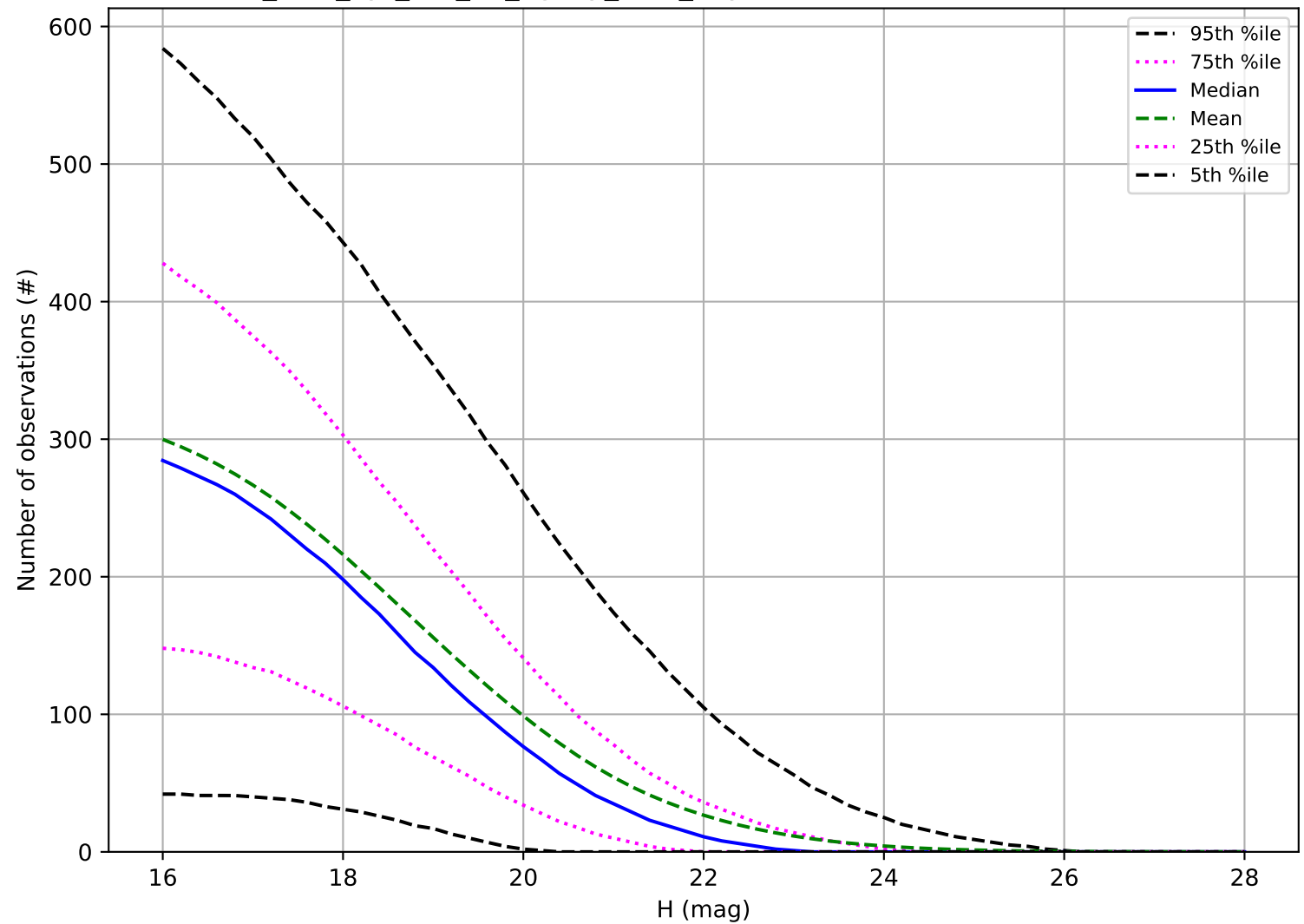
too_elab_2yr_r64_d3_ugrizy_v3.4_10yrs: Number of observations PHA
