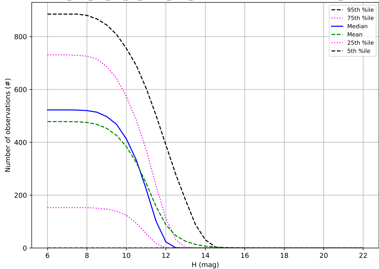
too_elab_2yr_r64_d3_ugrizy_v3.4_10yrs: Number of observations OCC_r20
