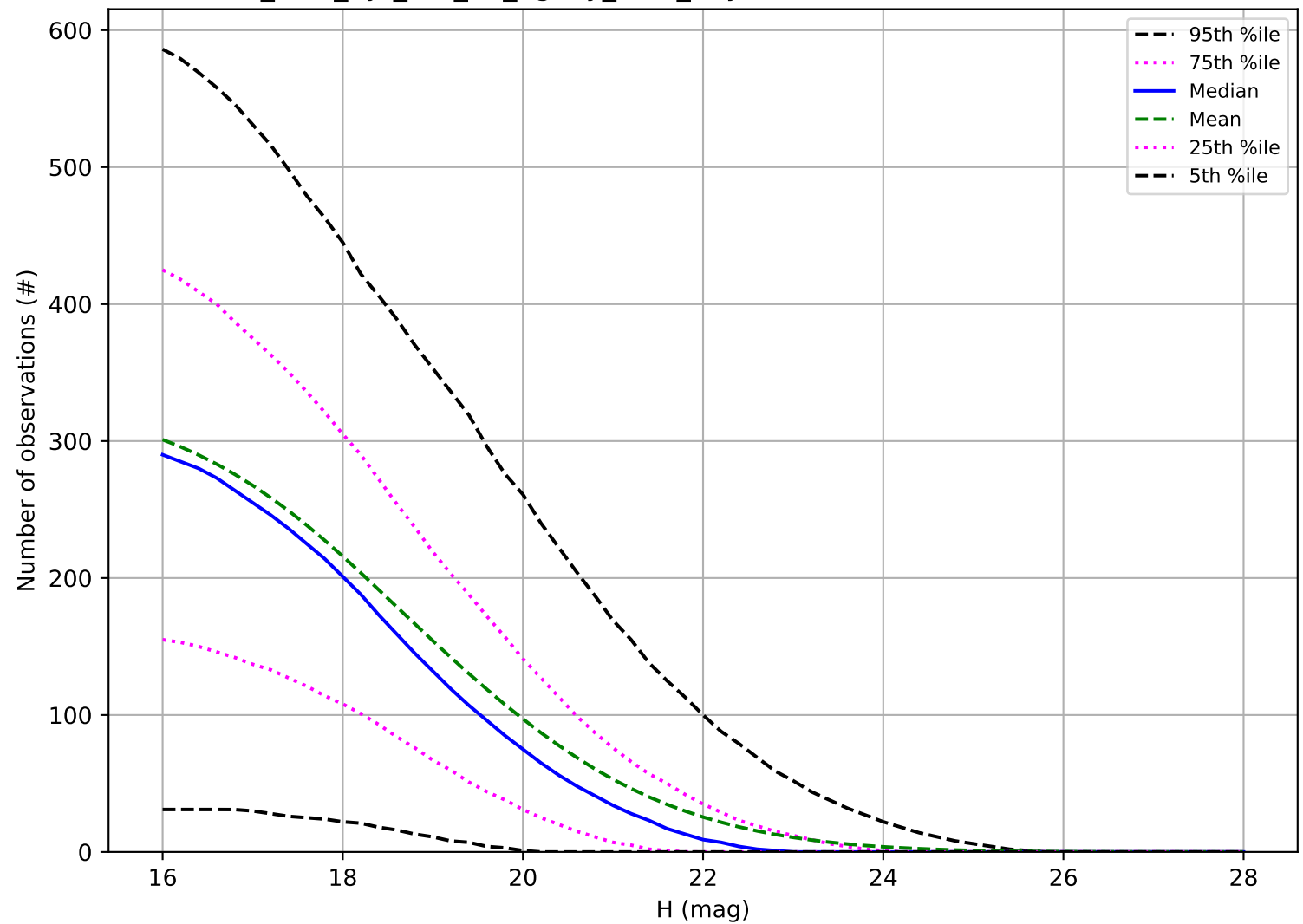
too_elab_2yr_r64_d3_ugrizy_v3.4_10yrs: Number of observations NEO
