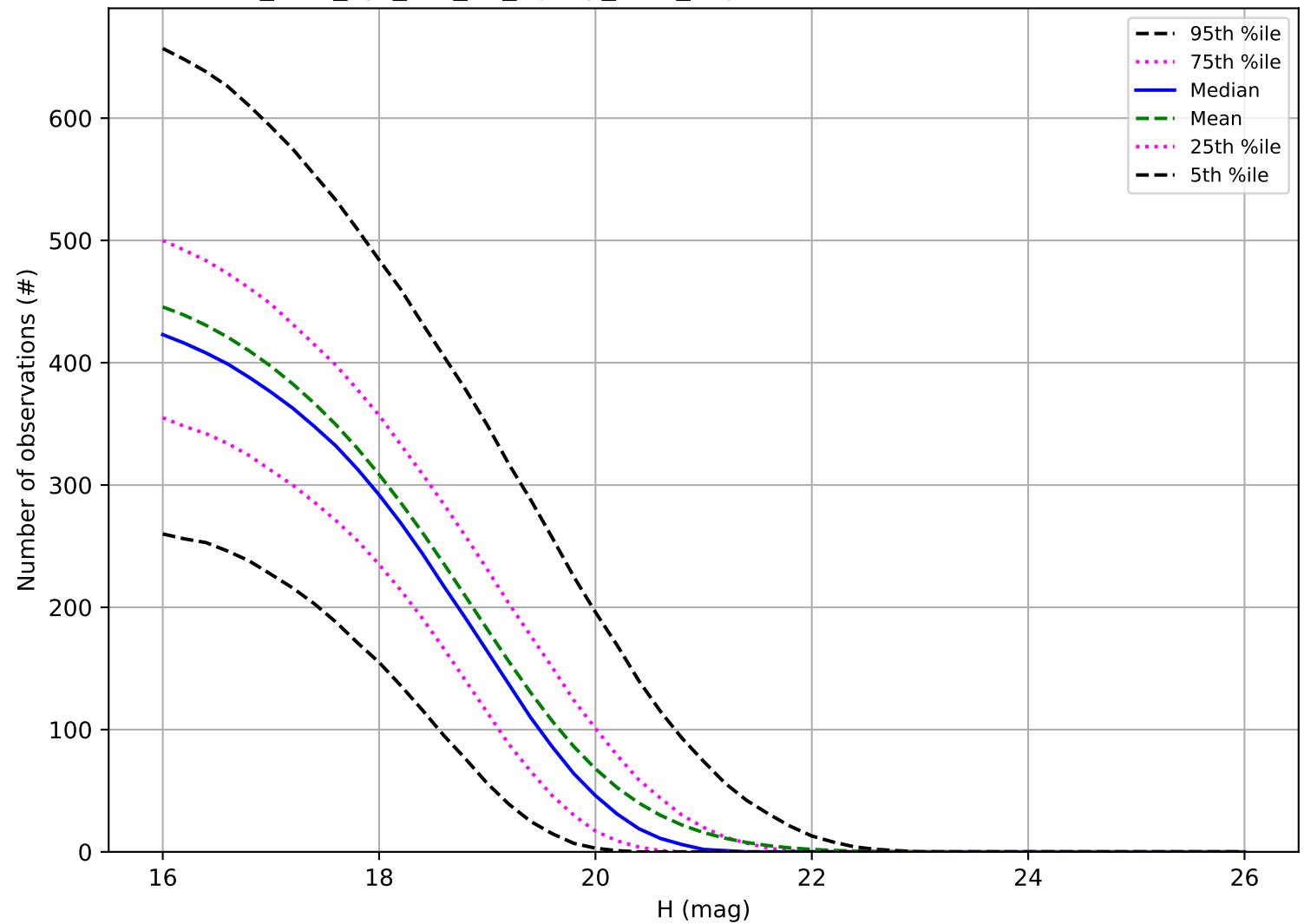
too_elab_2yr_r64_d3_ugrizy_v3.4_10yrs: Number of observations MBA
