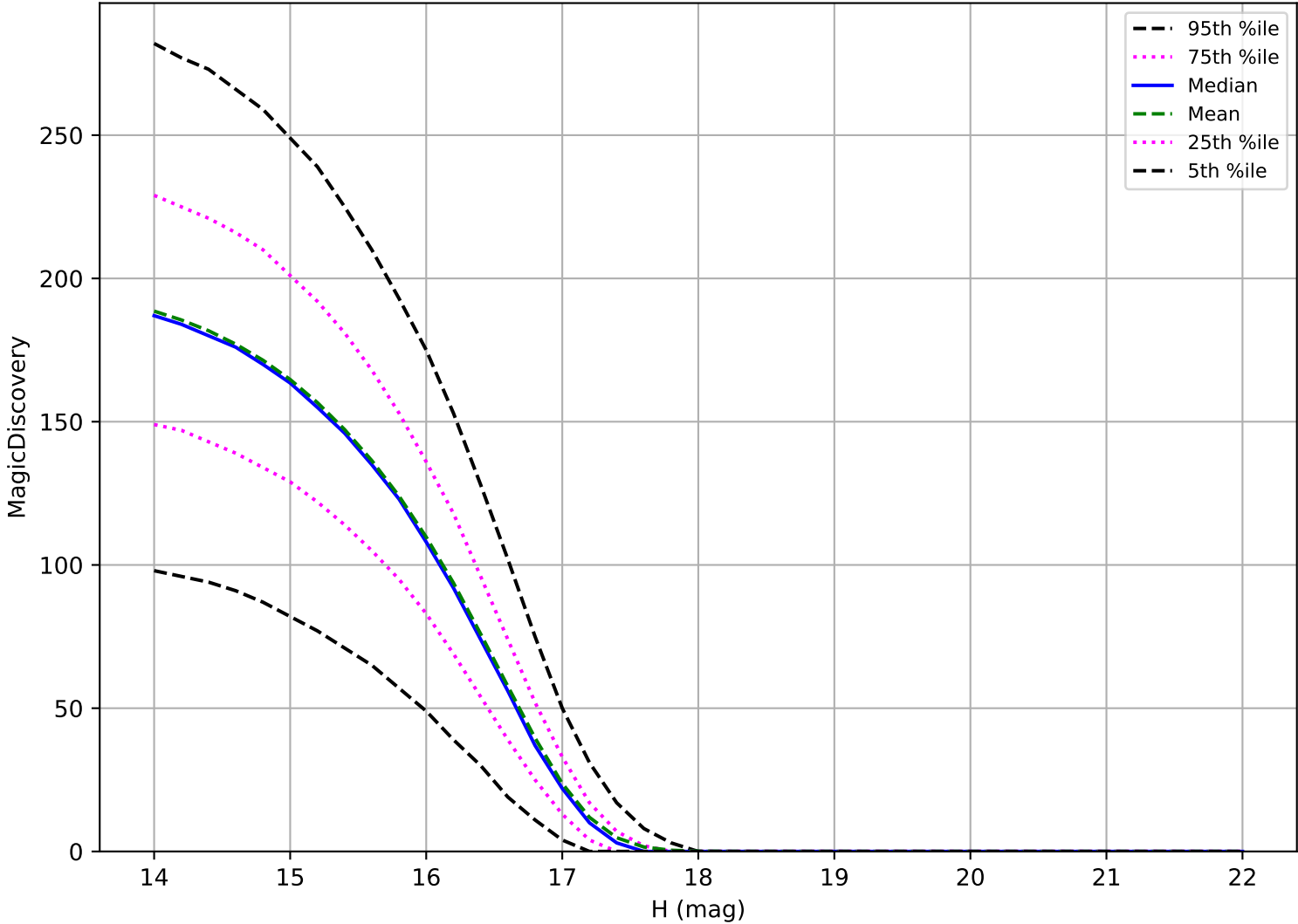
too_elab_2yr_r64_d3_ugrizy_v3.4_10yrs: Trojan 6 detections in 60 nights detection loss
