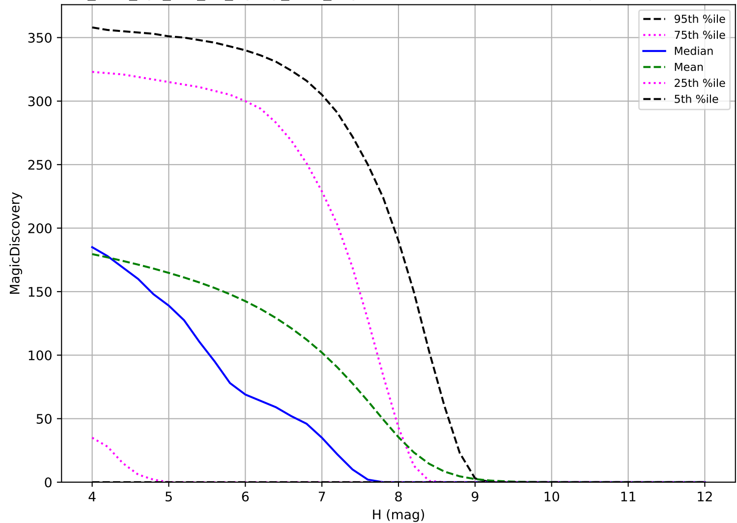
too_elab_2yr_r64_d3_ugrizy_v3.4_10yrs: TNO 6 detections in 60 nights detection loss
