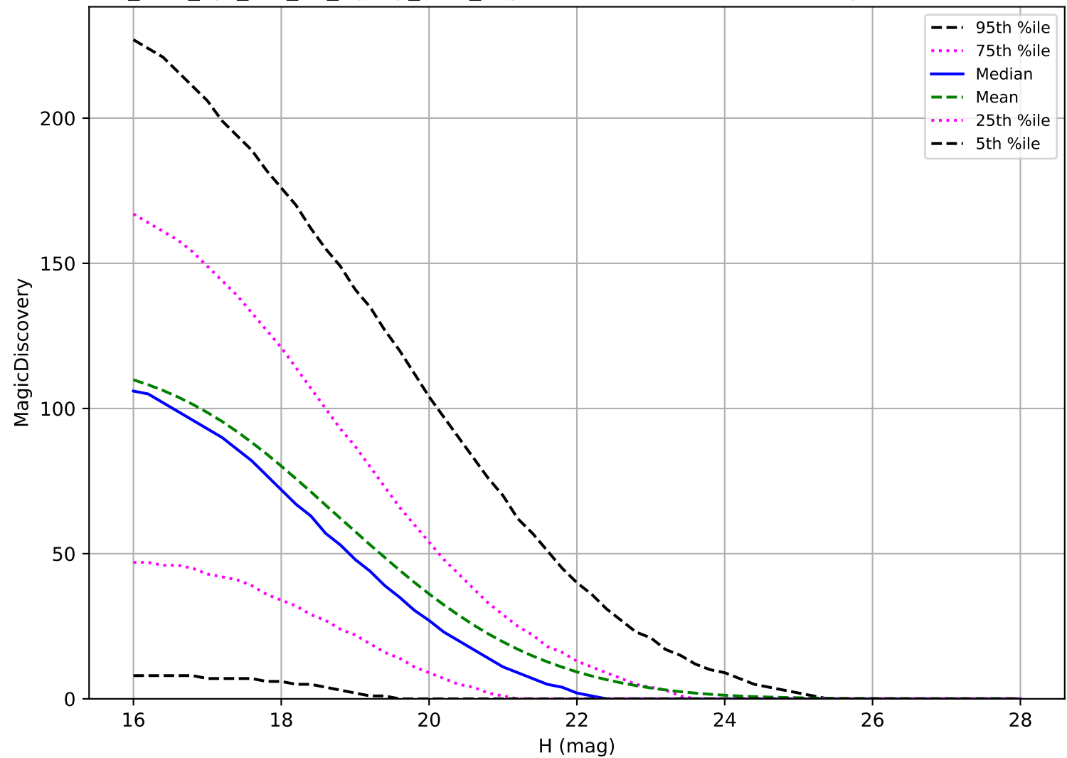
too_elab_2yr_r64_d3_ugrizy_v3.4_10yrs: PHA 6 detections in 60 nights detection loss
