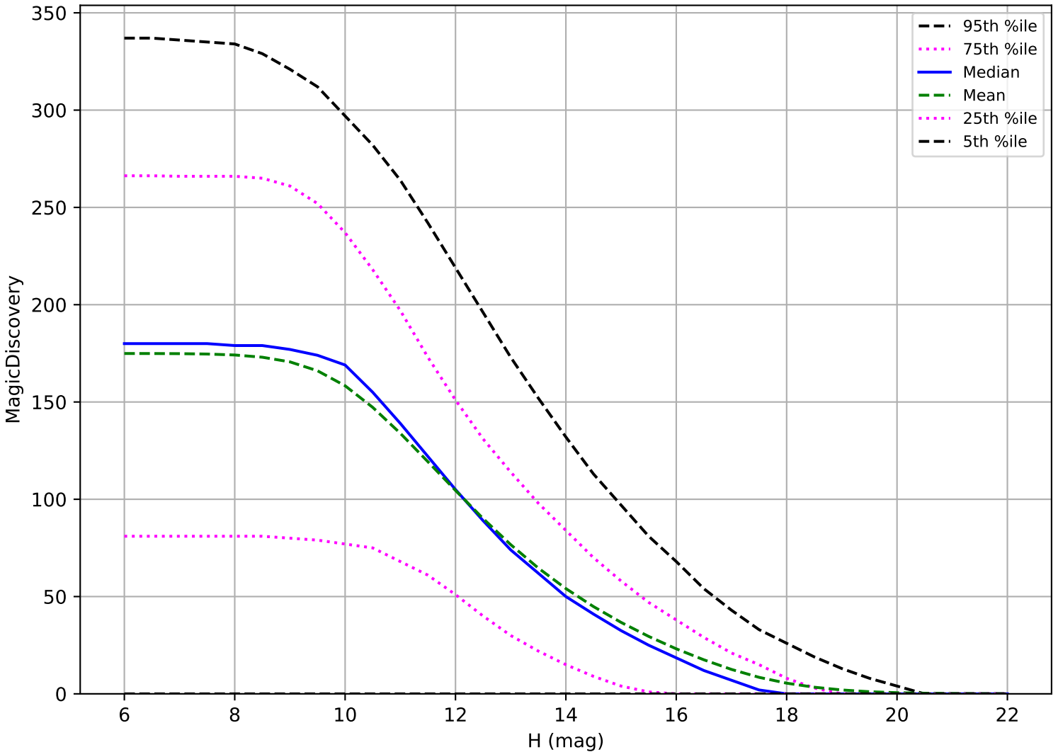
too_elab_2yr_r64_d3_ugrizy_v3.4_10yrs: OCC_r5 6 detections in 60 nights detection loss
