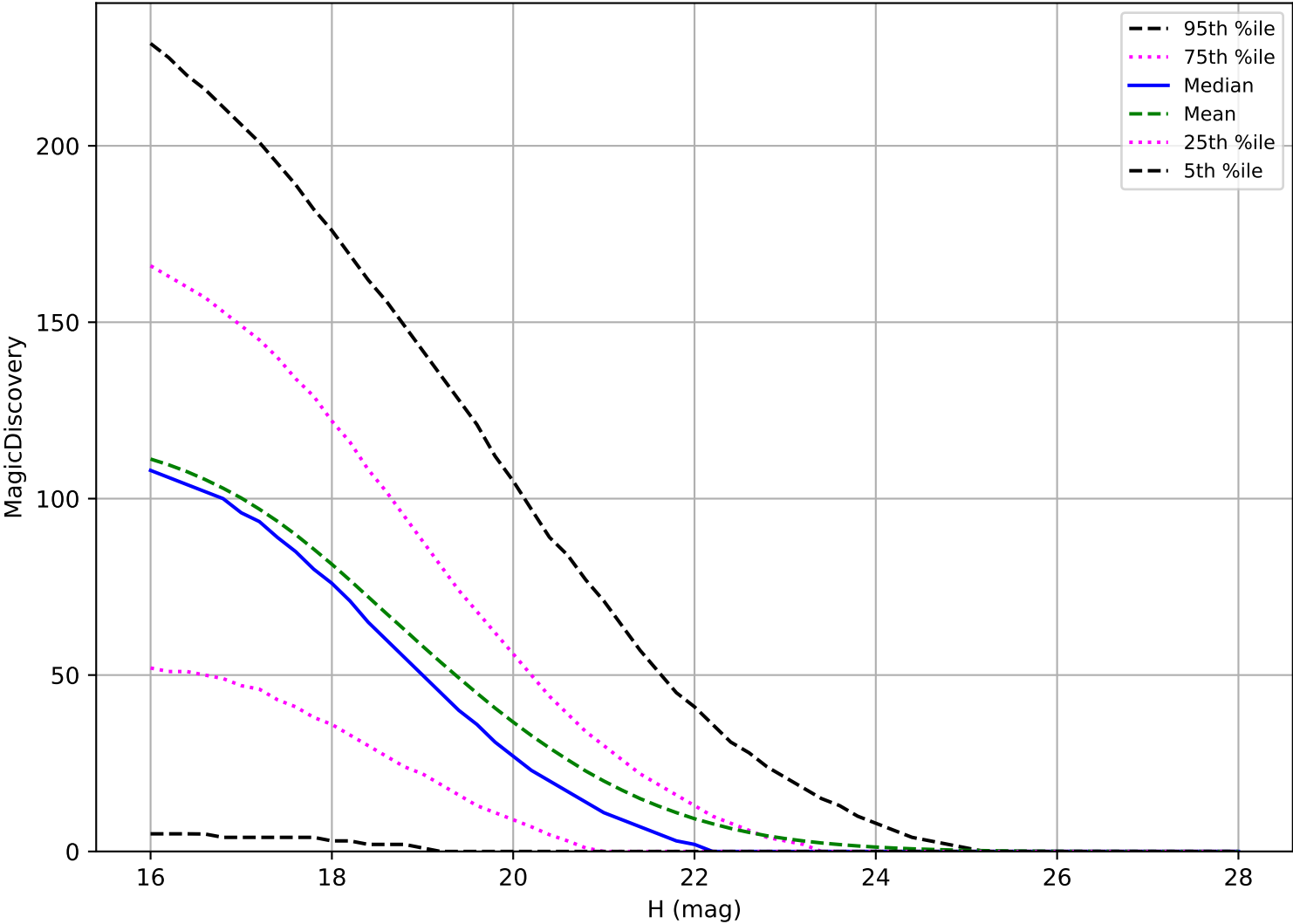
too_elab_2yr_r64_d3_ugrizy_v3.4_10yrs: NEO 6 detections in 60 nights detection loss
