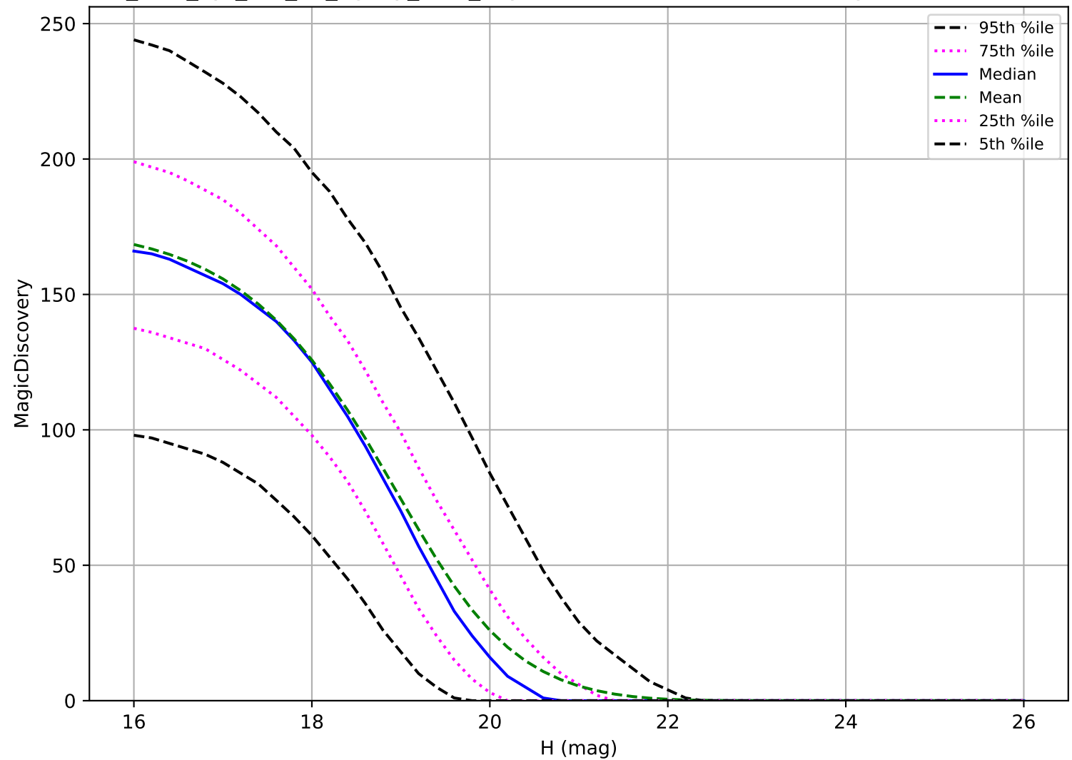
too_elab_2yr_r64_d3_ugrizy_v3.4_10yrs: MBA 6 detections in 60 nights detection loss
