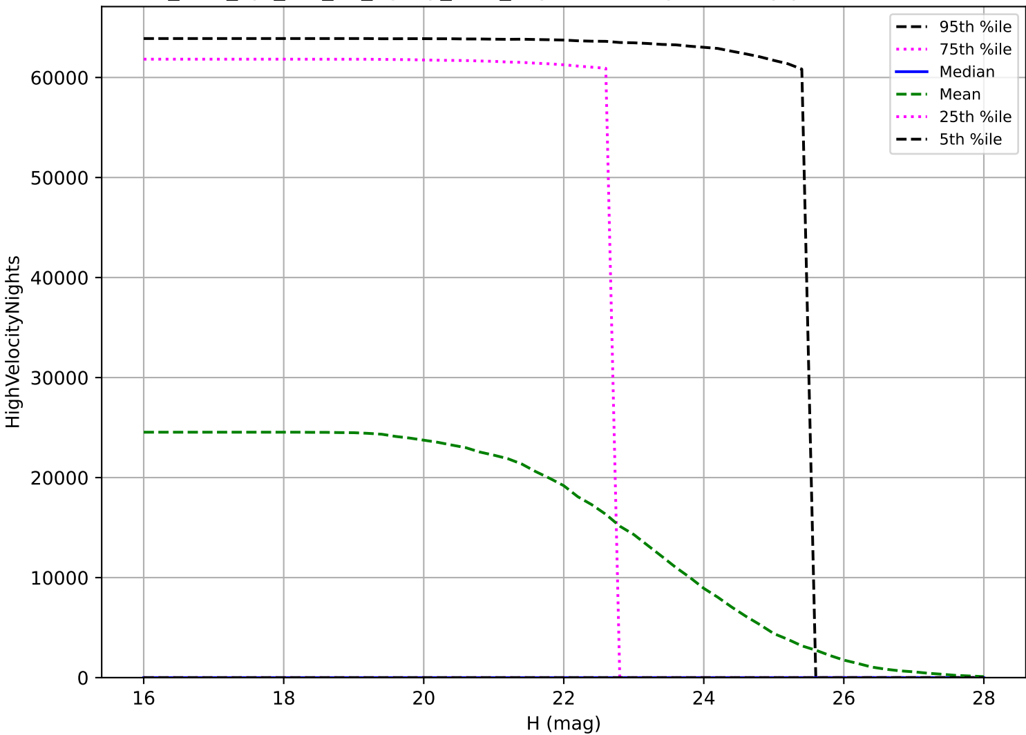
too_elab_2yr_r64_d3_ugrizy_v3.4_10yrs: PHA High velocity pair detection loss
