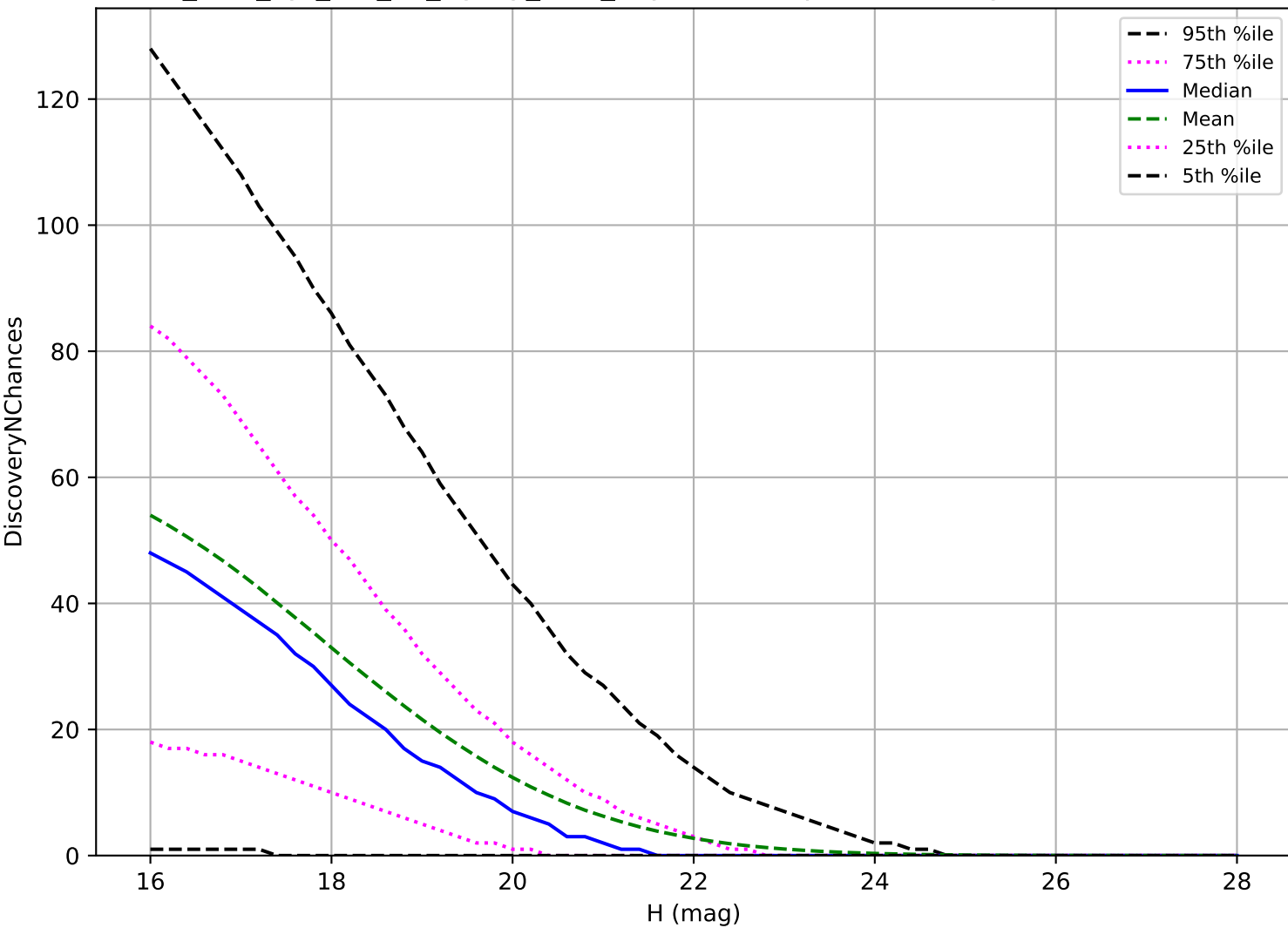
too_elab_2yr_r64_d3_ugrizy_v3.4_10yrs: PHA 3 pairs in 15 nights detection loss
