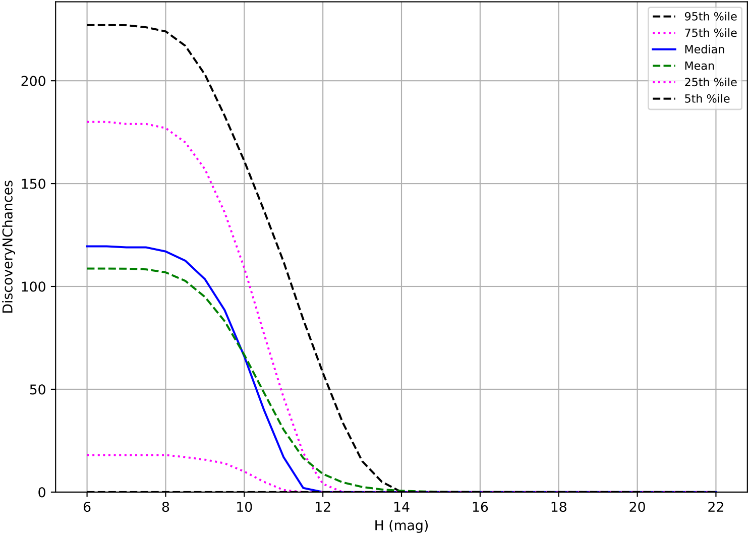
too_elab_2yr_r64_d3_ugrizy_v3.4_10yrs: OCC_r20 3 pairs in 15 nights detection loss
