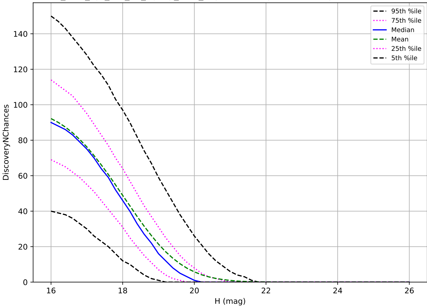
too_elab_2yr_r64_d3_ugrizy_v3.4_10yrs: MBA 3 pairs in 15 nights detection loss
