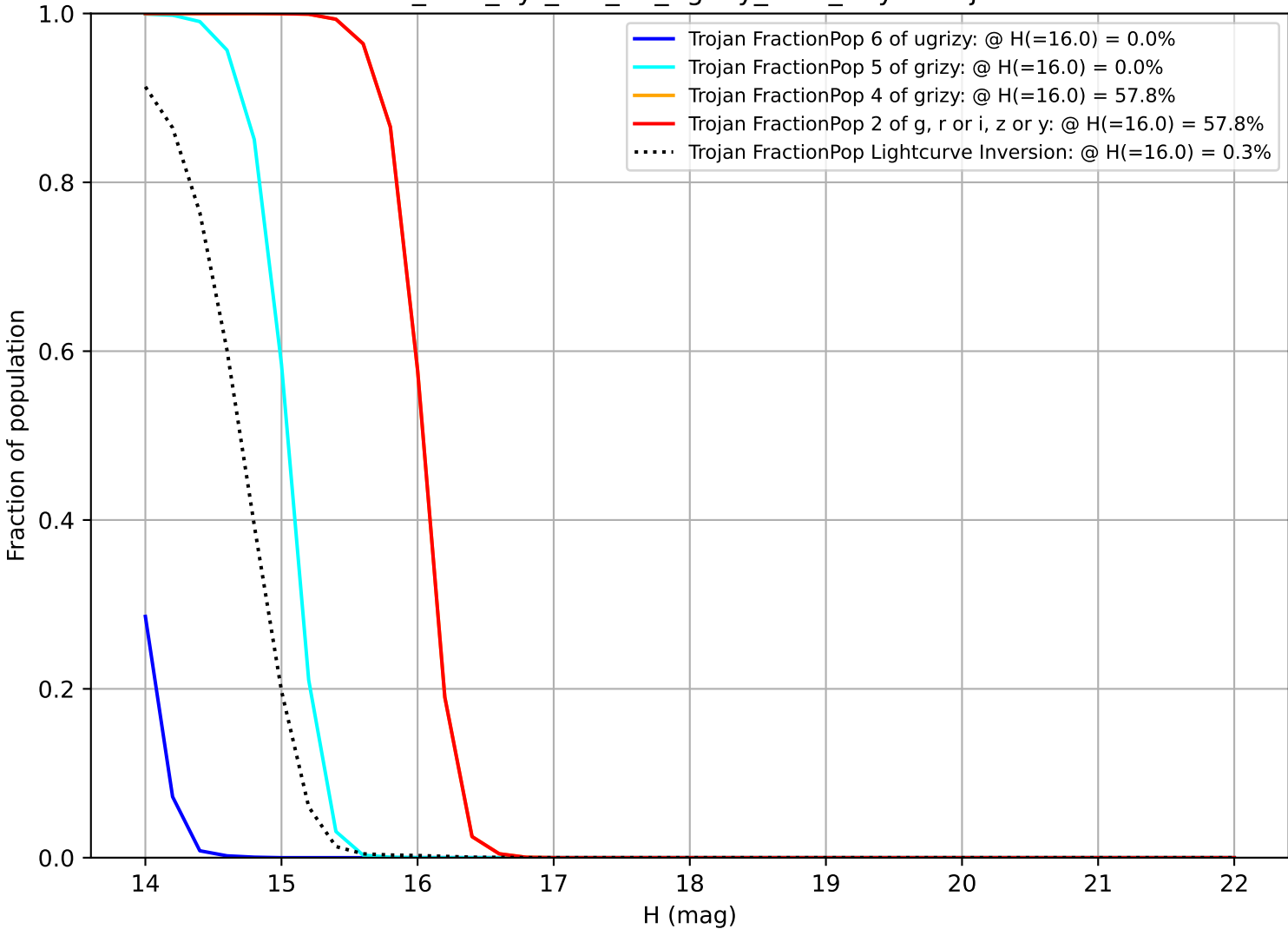
too_elab_2yr_r64_d3_ugrizy_v3.4_10yrs Trojan
