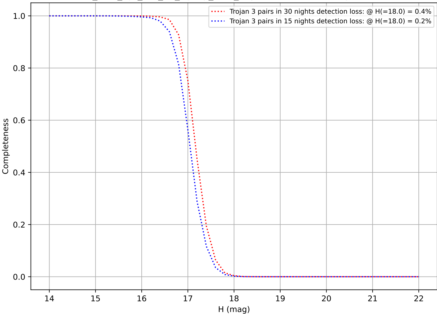
too_elab_2yr_r64_d3_ugrizy_v3.4_10yrs: DifferentialCompleteness
