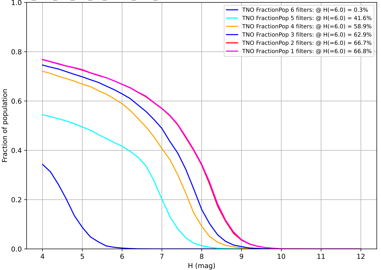
too_elab_2yr_r64_d3_ugrizy_v3.4_10yrs: Fraction of population with colors in X filters TNO
