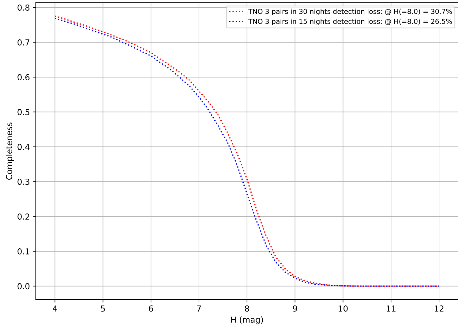
too_elab_2yr_r64_d3_ugrizy_v3.4_10yrs: DifferentialCompleteness
