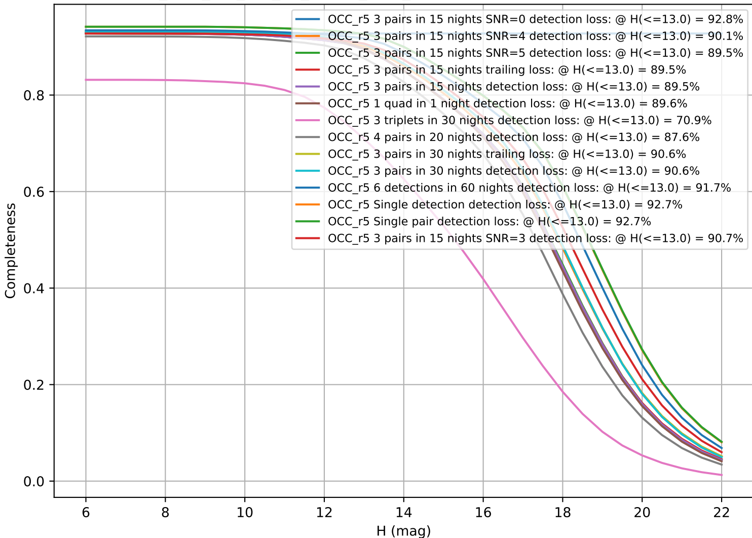
too_elab_2yr_r64_d3_ugrizy_v3.4_10yrs: CumulativeCompleteness
