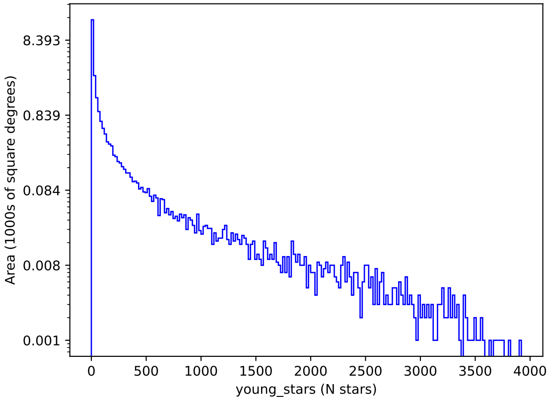
too_elab_2yr_r64_d3_ugrizy_v3.4_10yrs : young_stars
