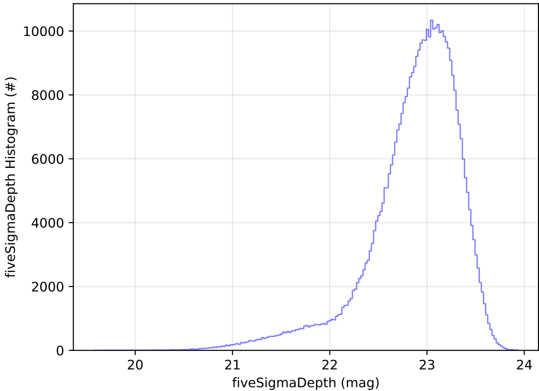
too_elab_2yr_r64_d3_ugrizy_v3.4_10yrs z: fiveSigmaDepth Histogram
