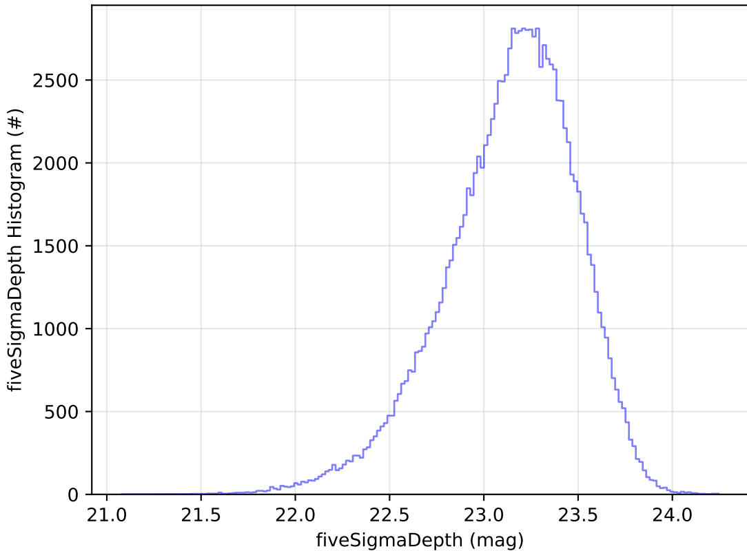
too_elab_2yr_r64_d3_ugrizy_v3.4_10yrs u: fiveSigmaDepth Histogram
