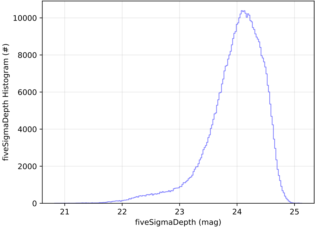
too_elab_2yr_r64_d3_ugrizy_v3.4_10yrs r: fiveSigmaDepth Histogram
