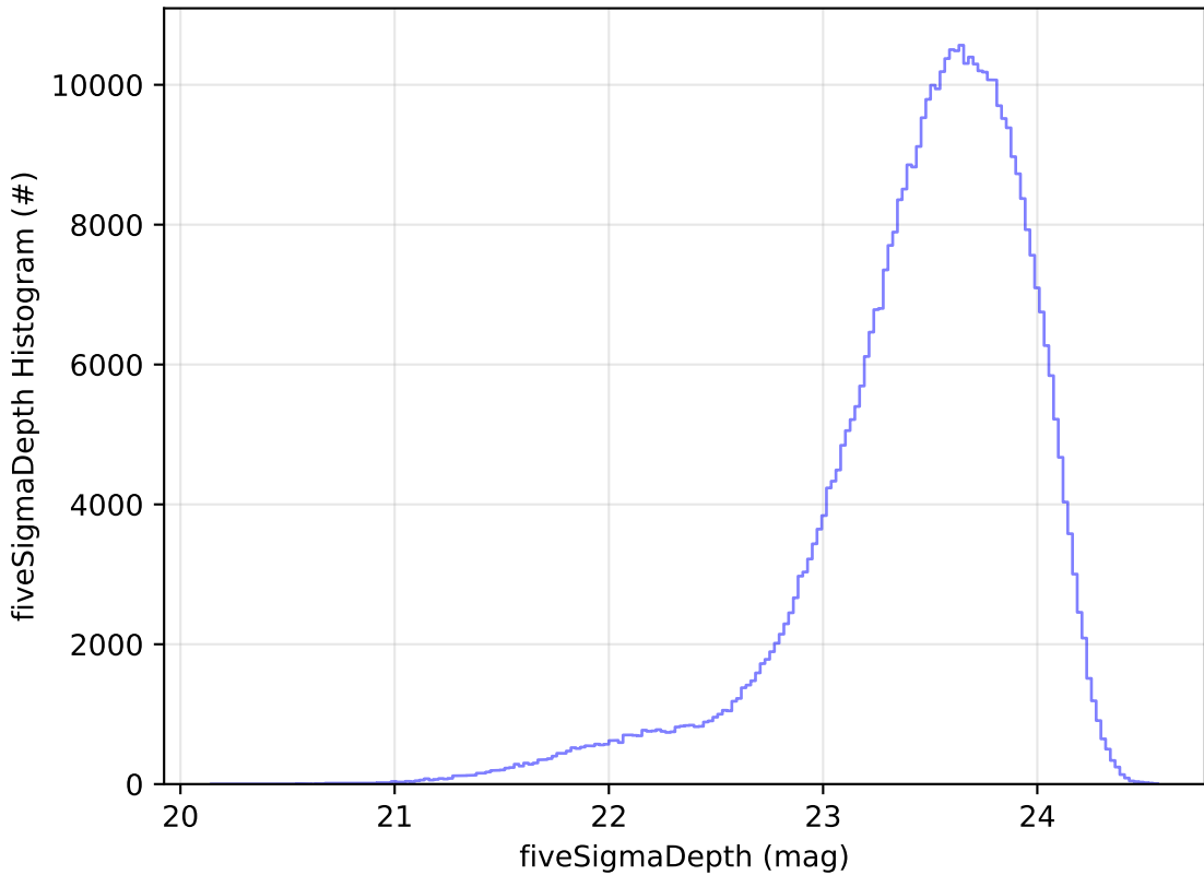
too_elab_2yr_r64_d3_ugrizy_v3.4_10yrs i: fiveSigmaDepth Histogram
