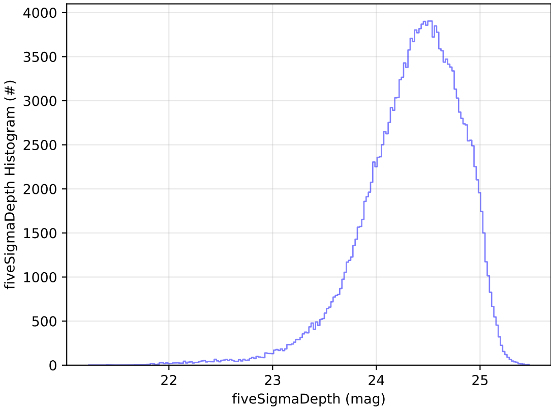
too_elab_2yr_r64_d3_ugrizy_v3.4_10yrs g: fiveSigmaDepth Histogram
