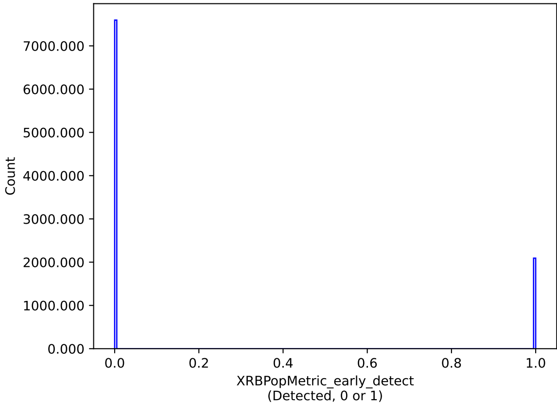
too_elab_2yr_r64_d3_ugrizy_v3.4_10yrs : XRBPoMetric_early_detect
