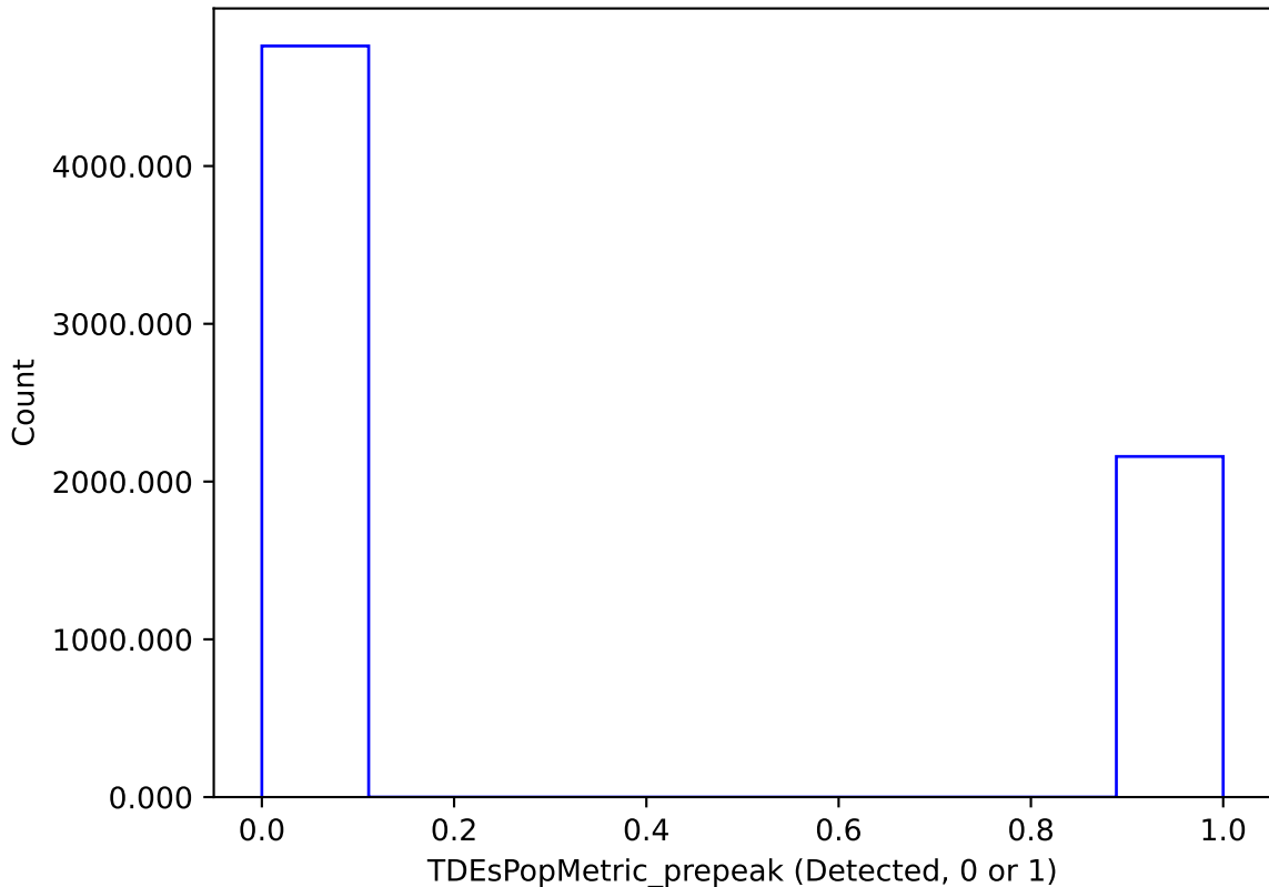
too_elab_2yr_r64_d3_ugrizy_v3.4_10yrs : TDEsPopMetric_prepeak
