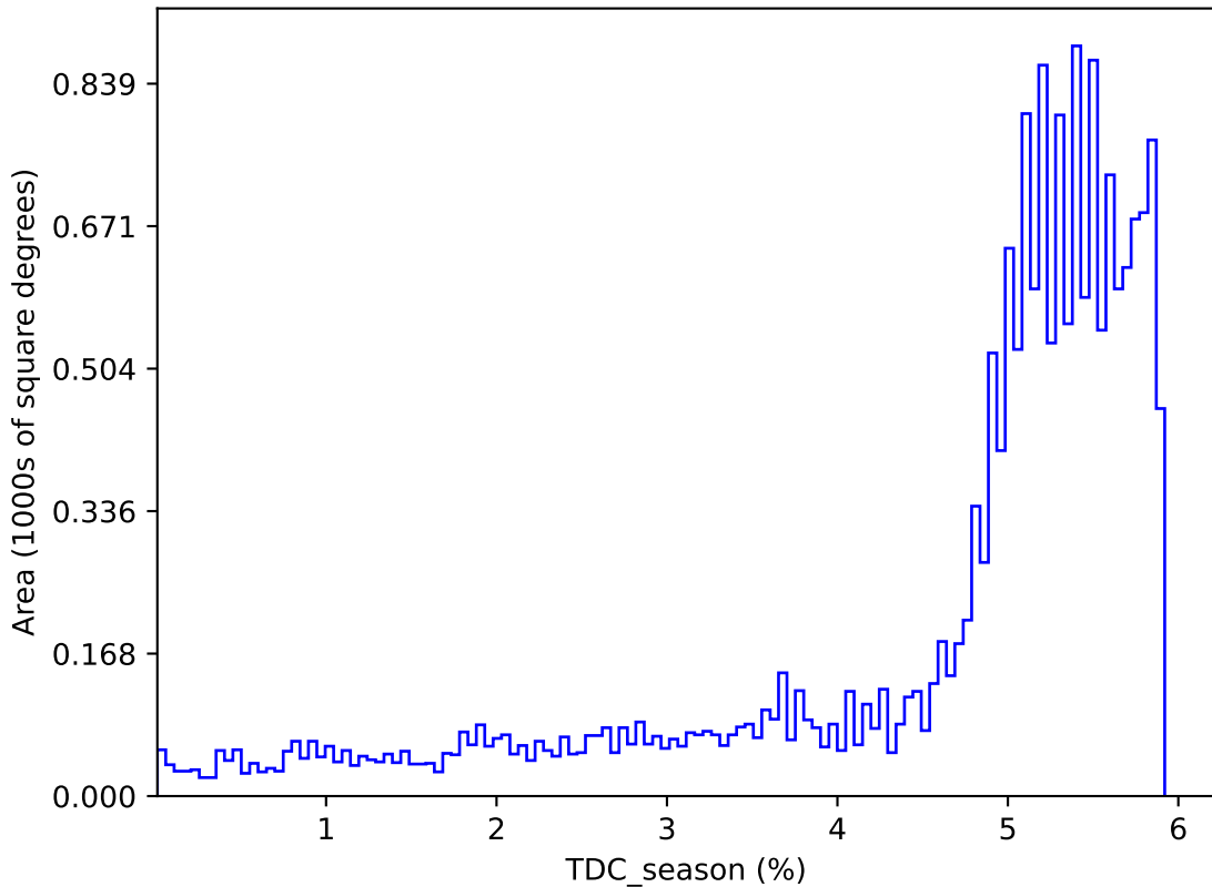
too_elab_2yr_r64_d3_ugrizy_v3.4_10yrs : TDC_season
