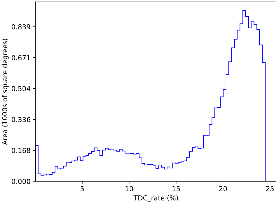
too_elab_2yr_r64_d3_ugrizy_v3.4_10yrs : TDC_rate
