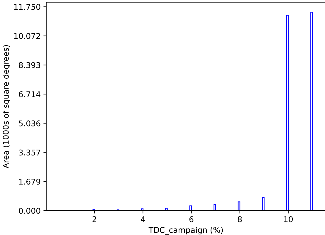
too_elab_2yr_r64_d3_ugrizy_v3.4_10yrs : TDC_campaign
