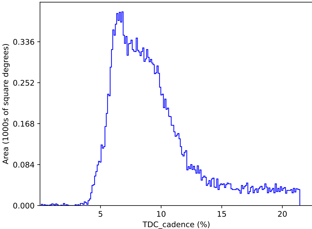
too_elab_2yr_r64_d3_ugrizy_v3.4_10yrs : TDC_cadence
