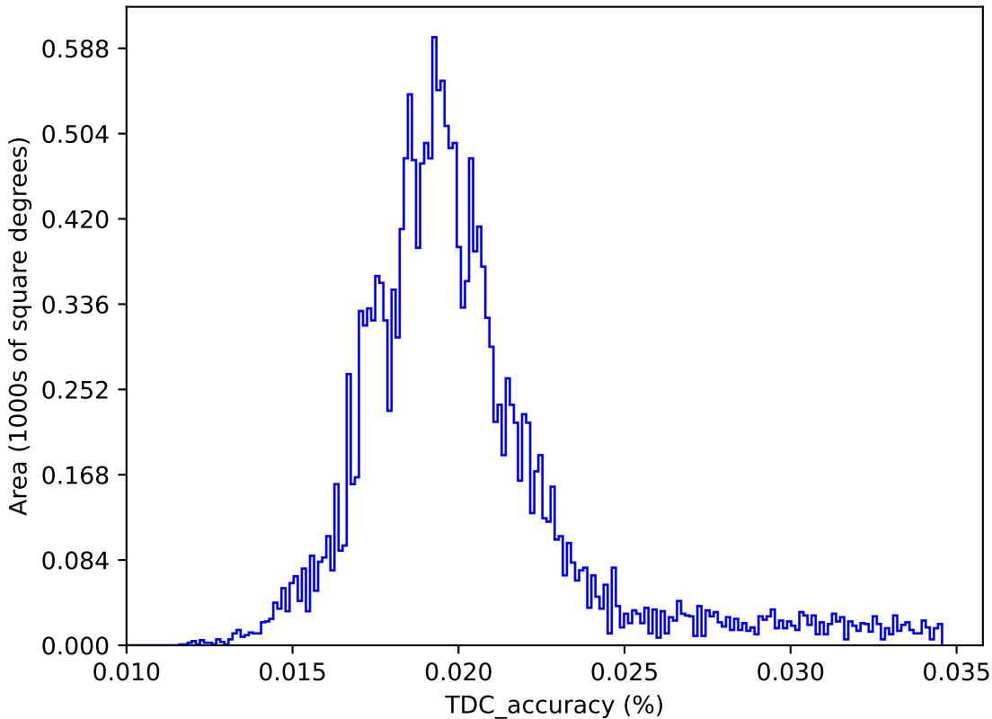
too_elab_2yr_r64_d3_ugrizy_v3.4_10yrs : TDC_accuracy
