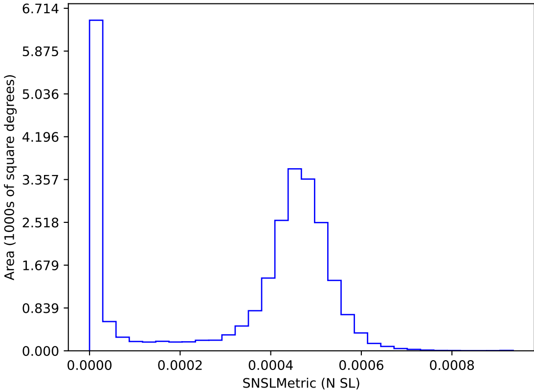
too_elab_2yr_r64_d3_ugrizy_v3.4_10yrs : SNSLMetric
