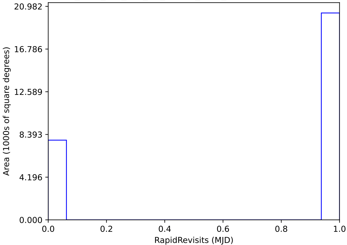
too_elab_2yr_r64_d3_ugrizy_v3.4_10yrs : RapidRevisits
