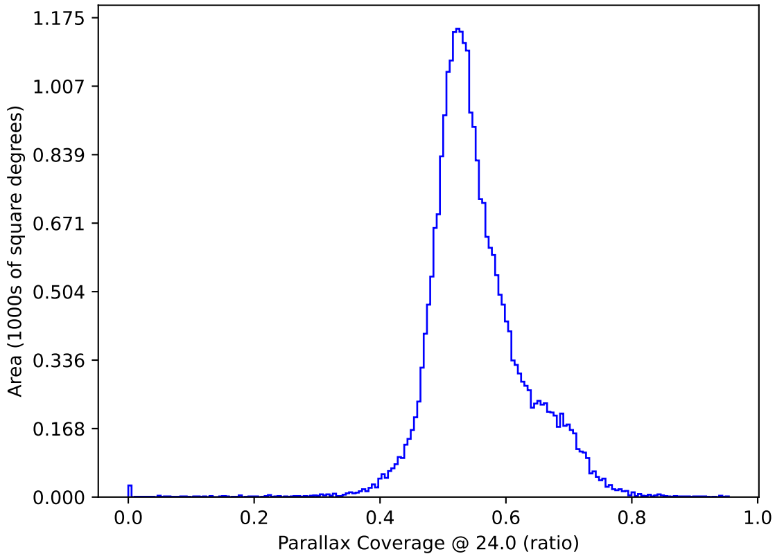
too_elab_2yr_r64_d3_ugrizy_v3.4_10yrs : Parallax Coverage @ 24.0
