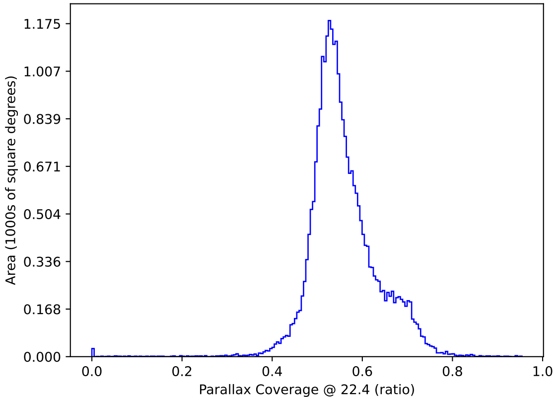
too_elab_2yr_r64_d3_ugrizy_v3.4_10yrs : Parallax Coverage @ 22.4
