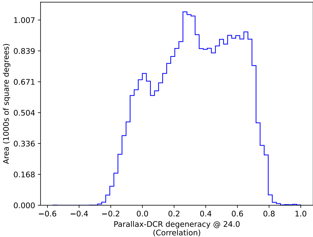
too_elab_2yr_r64_d3_ugrizy_v3.4_10yrs : Parallax-DCR degeneracy @ 24.0
