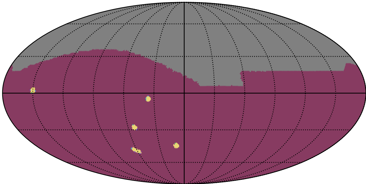
too_elab_2yr_r64_d3_ugrizy_v3.4_10yrs : NumberOfQuickRevisits
