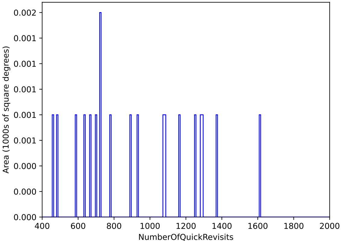
too_elab_2yr_r64_d3_ugrizy_v3.4_10yrs : NumberOfQuickRevisits
