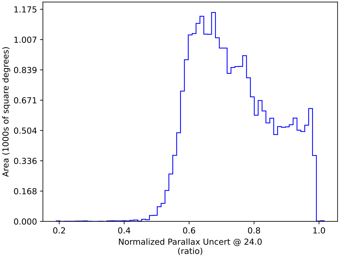
too_elab_2yr_r64_d3_ugrizy_v3.4_10yrs : Normalized Parallax Uncert @ 24.0
