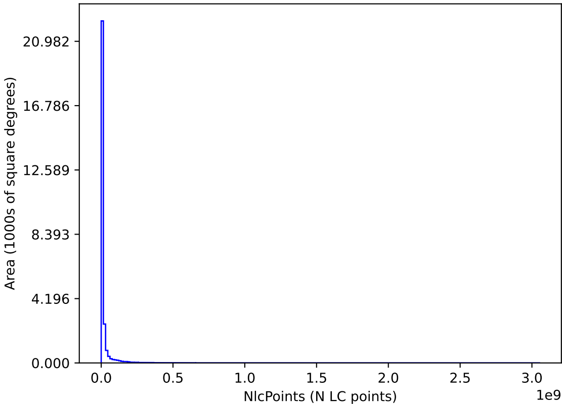
too_elab_2yr_r64_d3_ugrizy_v3.4_10yrs : NlcPoints
