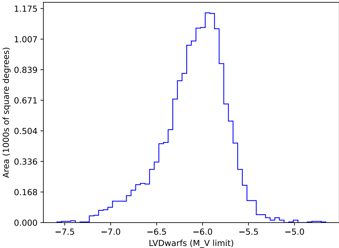
too_elab_2yr_r64_d3_ugrizy_v3.4_10yrs gi: LVDwarfs
