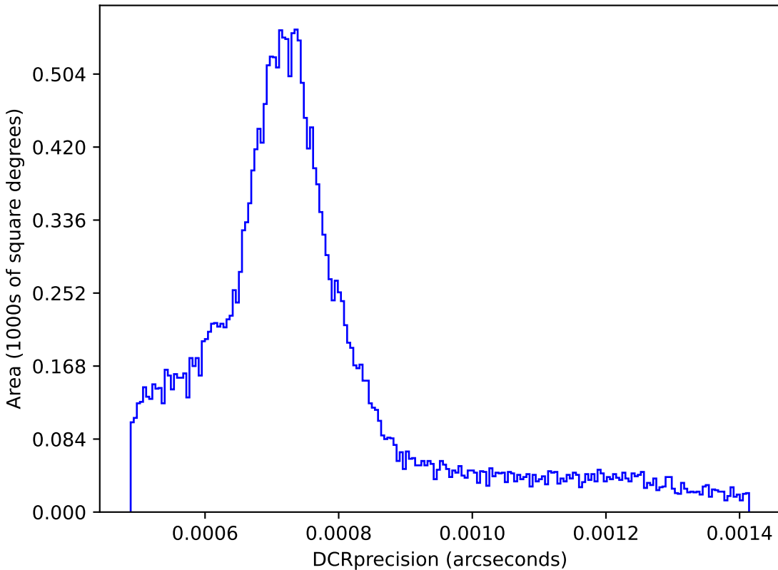
too_elab_2yr_r64_d3_ugrizy_v3.4_10yrs : DCRprecision
