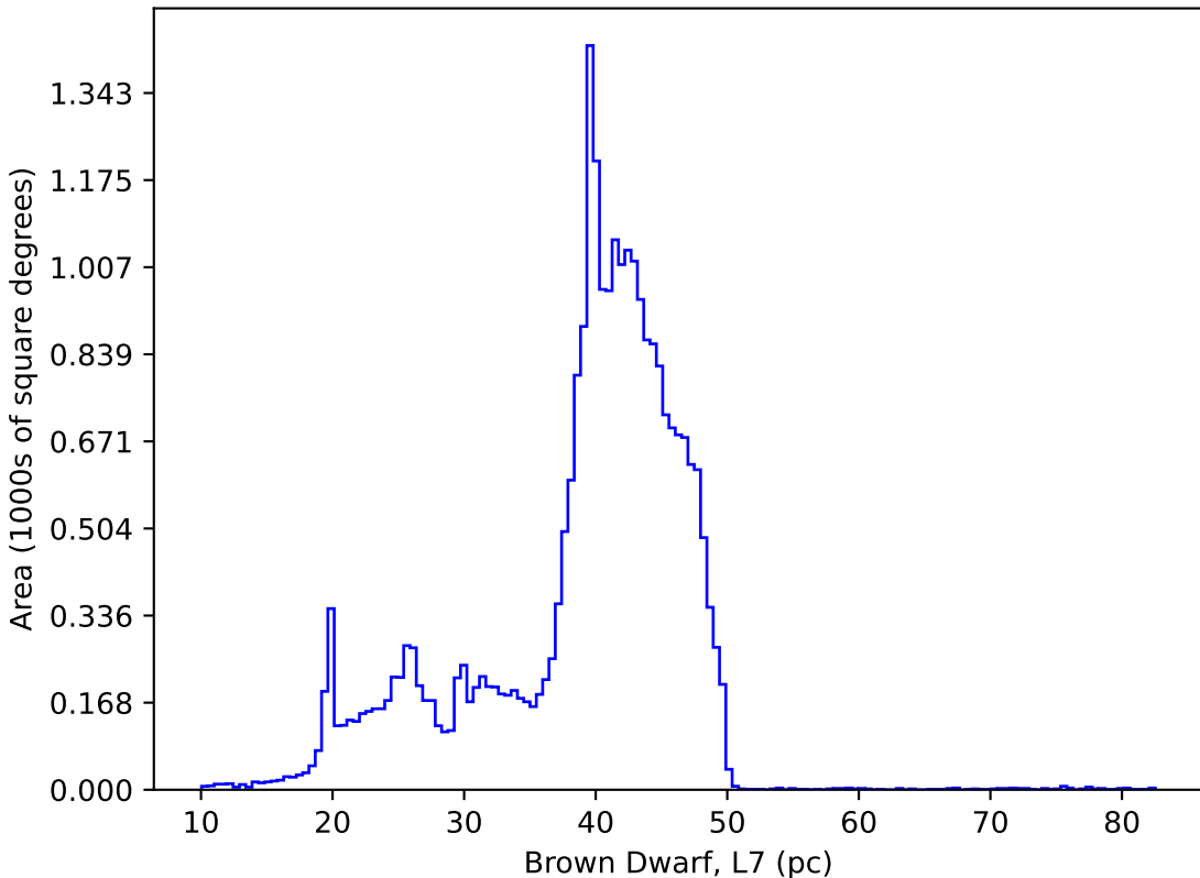
too_elab_2yr_r64_d3_ugrizy_v3.4_10yrs : Brown Dwarf, L7
